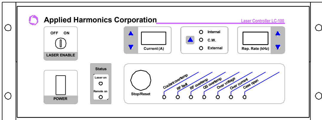
Figure The LC-100 power supply / controller front panel.
